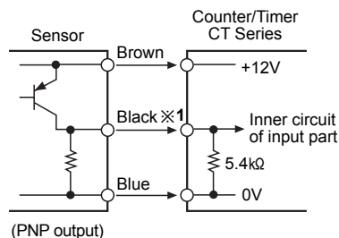
(PNP output)
