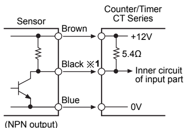
(NPN output)
