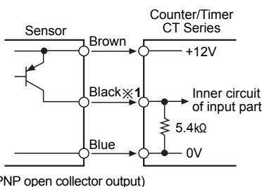
(PNP open collector output)
